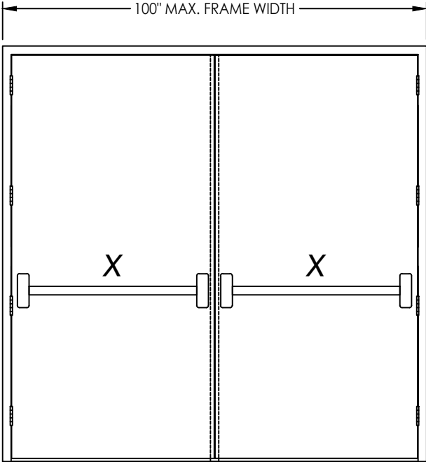
PANIC BAR EXIT DEVICE w/ REMOVABLE MULLION
