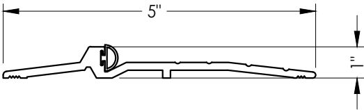
5 OUTSWING BUMP THRESHOLD HAGER 520S
