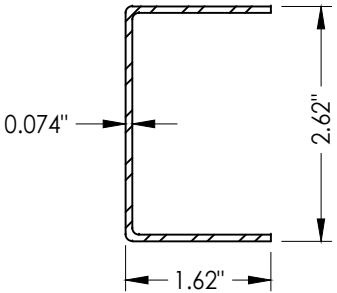
3 MULLION REINFORCEMENT
