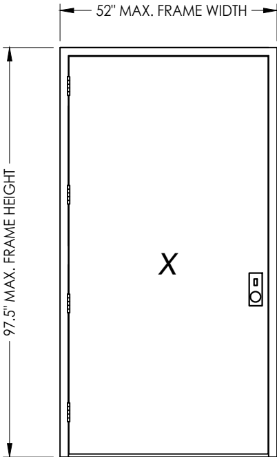
MORTISE LOCK & DEADBOLT
