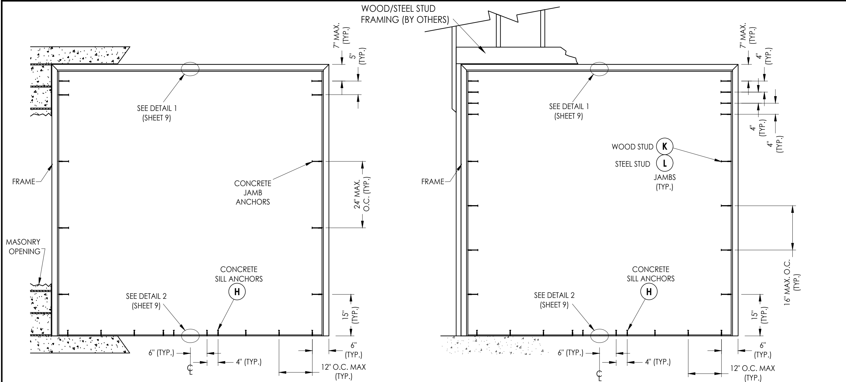
FRAME ANCHORING Masonry Construction Concrete Anchors
